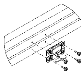
A (1:5)
